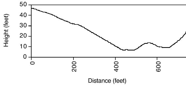
Figure 12 Elevation profile along shadow cast by object 5.
